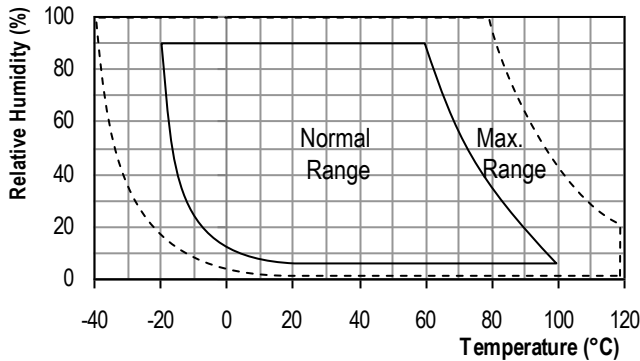
Figure 4 Operating Conditions
