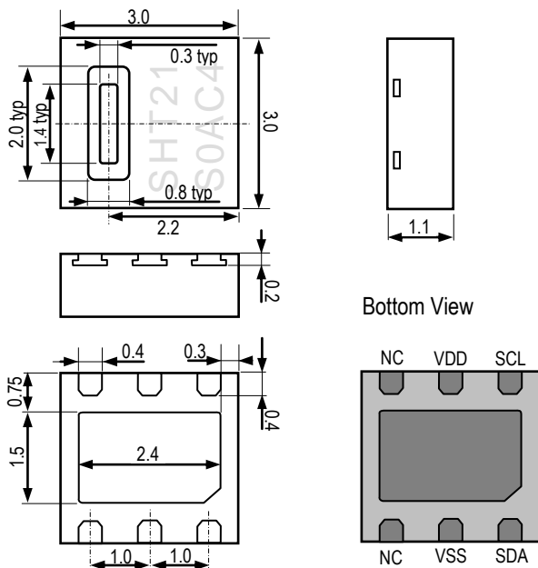
Figure 1: Drawing of SHT21S sensor package, dimensions are given in mm (1mm = 0.039inch), tolerances are \pm 0.1 mm. The die pad (center pad) is internally connected to VSS. The NC pads must be left floating. Numbering of E/O pads starts at lower right corner (indicated by notch in die pad) and goes clockwise (compare Table 2).
