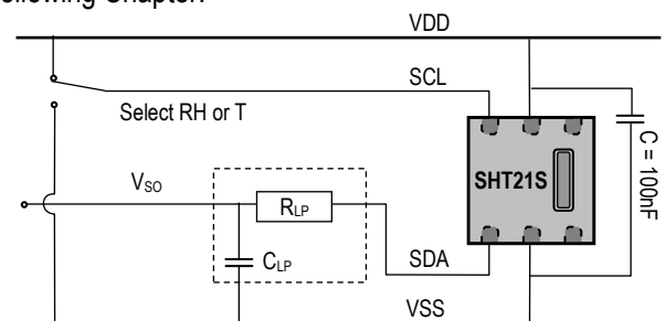
Figure 11 Typical circuit with low pass filter (surrounded by hatched line) for analog output. Recommended component size: R_{LP} = 100\text{k}\Omega and C_{LP} = 220\text{nF} . By pulling SCL low or high, the output value is switched to temperature or humidity, respectively.
